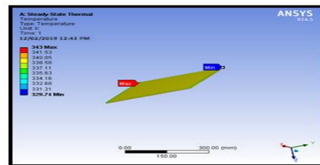
Fig47: Temperature distribution
