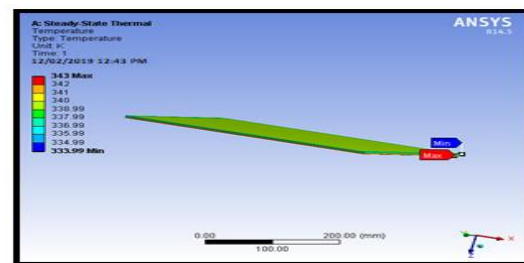
Fig 35 :Temperature distribution
